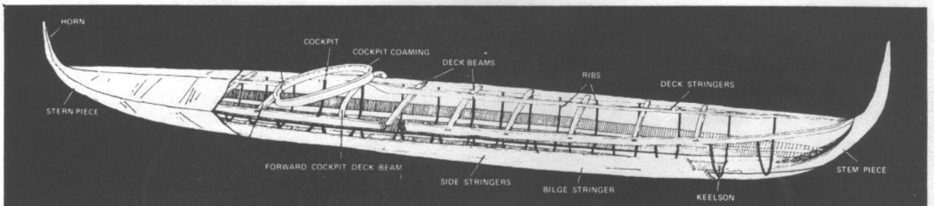
FIG. 2 — CONSTRUCTION DETAIL
